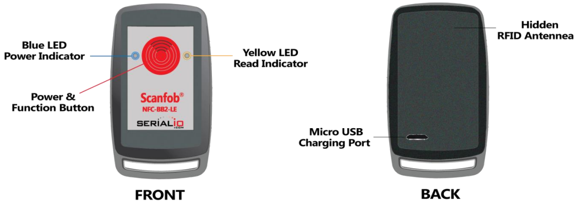
Figure 1: Scanfob® NFC-BB2e Layout
